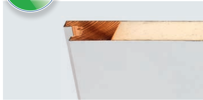
High thermal insulation thanks to a door leaf that is 46 mm thick and infilled with CFC-free PU rigid foam.
